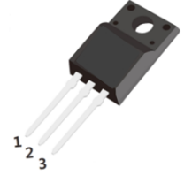
TO-220F(Ins)
