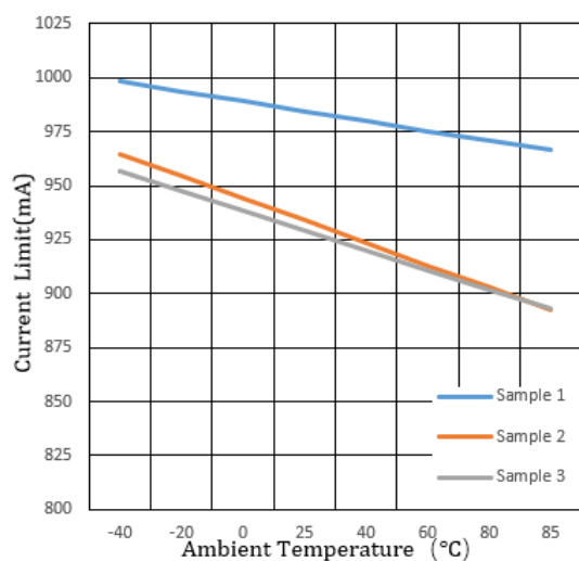
Current-Limit Threshold vs. Ambient Temperature
