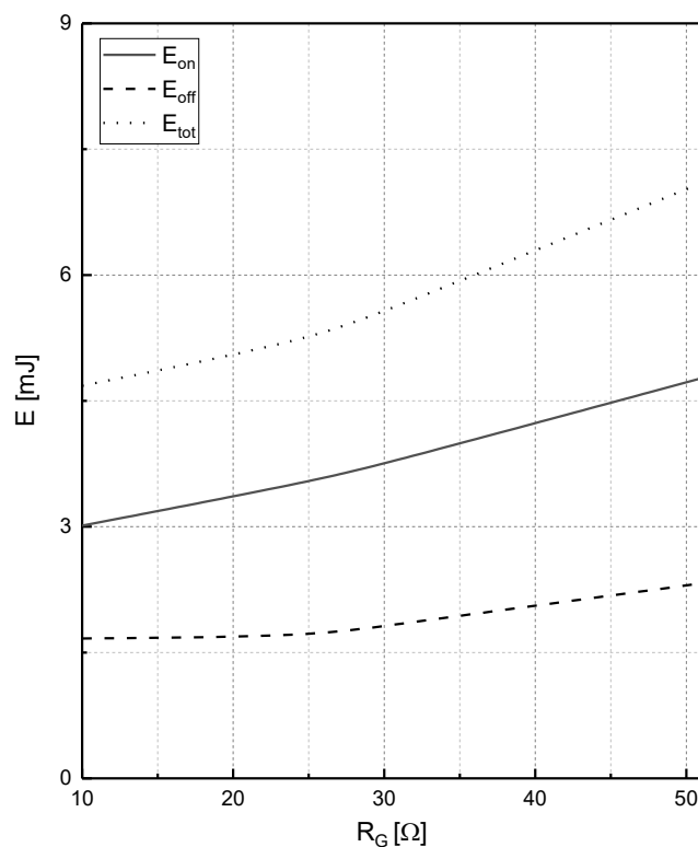
Fig.8 Typical switching energy losses as a function of R_G E=f(R_G) , V_{CC}=600V , I_C=40A , V_{GE}=0/15V , T_J=150^\circ C
