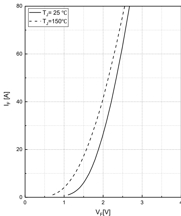
Fig.4 Typical I_F as a function of V_F
