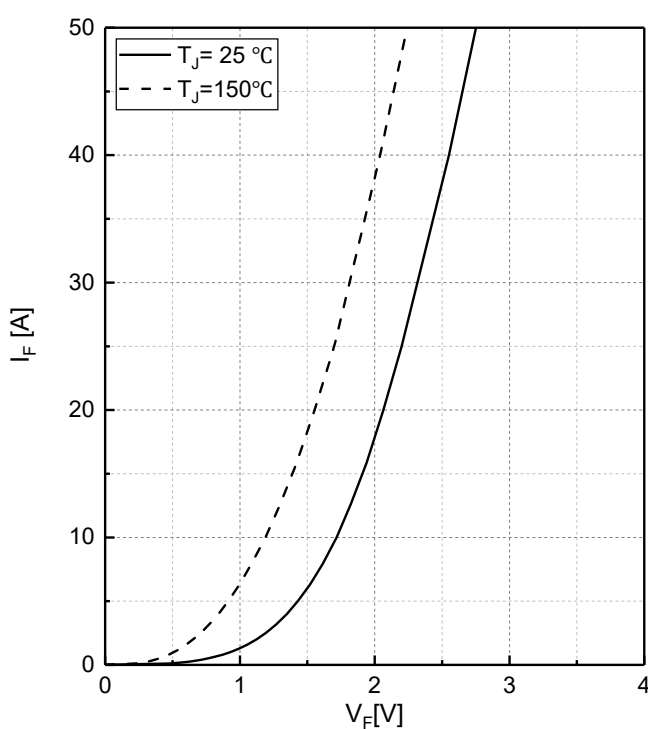
Fig.4 Typical I_F as a function of V_F I_F = f(V_F)
