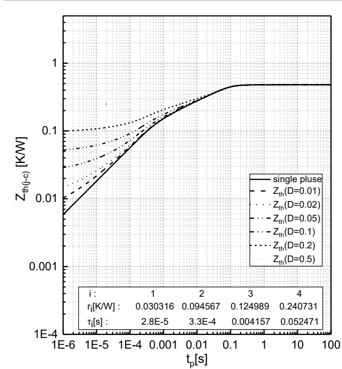
Fig.13 Transient thermal impedance of IGBT Z_{th(j-c)}=f(t_p) , D=t_p/T
