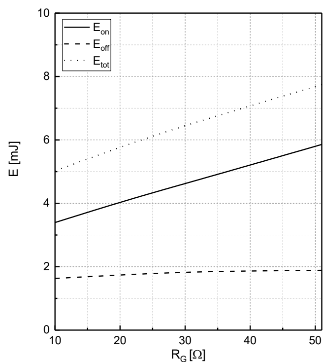
Fig.8 Typical switching energy losses as a function of R_G E=f(R_G) , V_{CC}=600V , I_C=25A , V_{GE}=0/15V , T_J=150^\circ C
