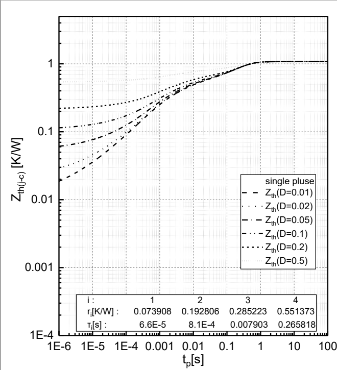
Fig.14 Transient thermal impedance of Diode Z_{th(j-c)}=f(t_p) , D=t_p/T
