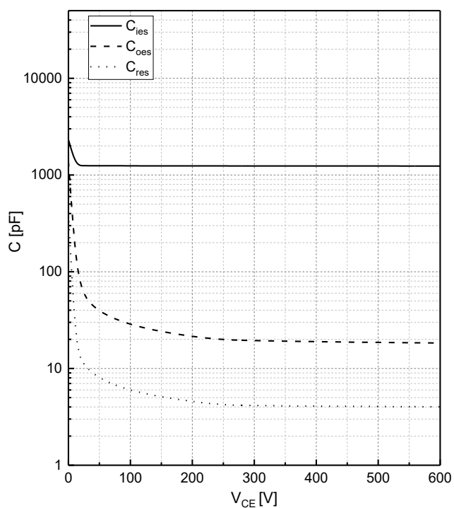
Fig.11 Typical capacitance as a function of V_{CE} C=f(V_{CE}) , f=1MHz , V_{GE}=0V
