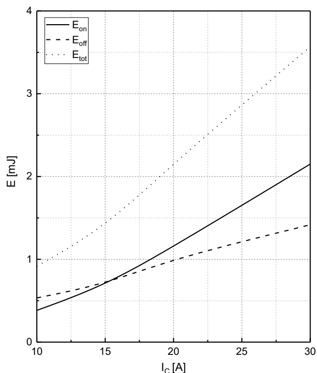
Fig.9 Typical switching energy losses as a function of I_C E=f(I_C) , V_{CC}=600V , R_G=10\Omega , V_{GE}=0/15V , T_J=150^\circ C
