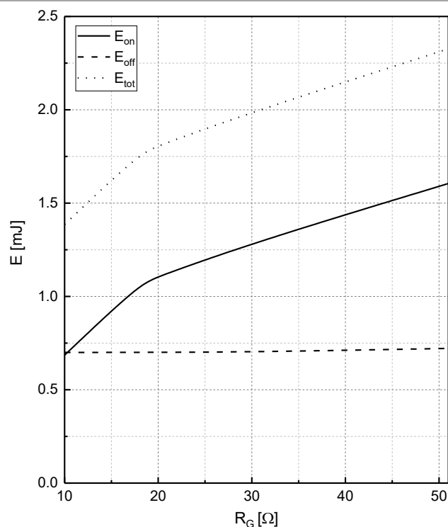
Fig.8 Typical switching energy losses as a function of R_G E=f(R_G) , V_{CC}=600V , I_C=15A , V_{GE}=0/15V , T_J=150^\circ C
