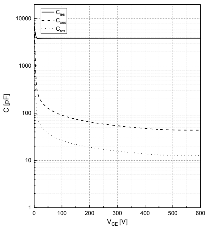
Fig.7 Typical capacitance as a function of V_{CE} C=f(V_{CE}) , f=1MHz , V_{GE}=0V
