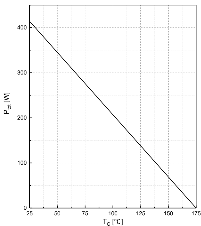
Fig.8 Power dissipation as a function of T_C P_{tot}=f(T_C) , T_{vj} \leq 175^\circ C
