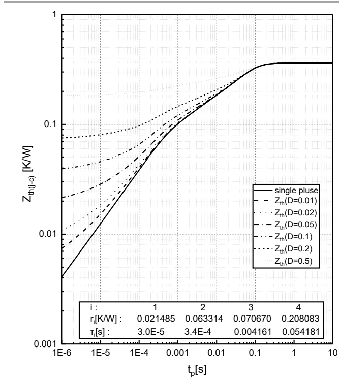
Fig.9 Transient thermal impedance of IGBT Z_{th(j-c)}=f(t_p), D=t_p/T
