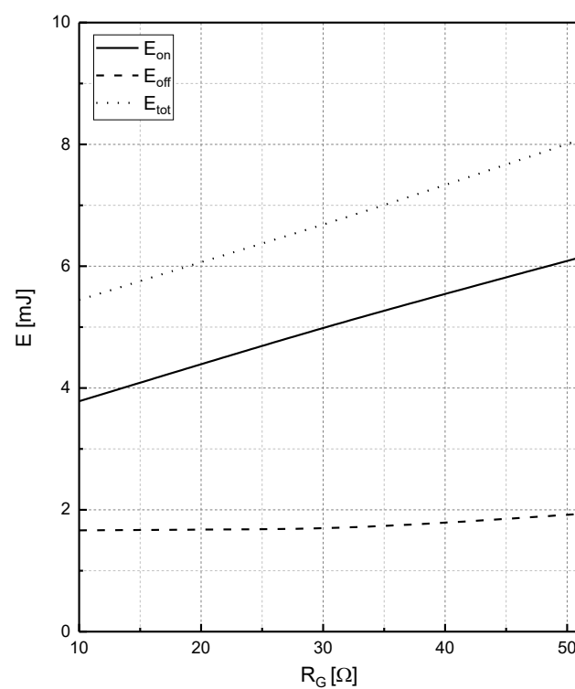
Fig.8 Typical switching energy losses as a function of R_G E=f(R_G) , V_{CC}=400V , I_C=75A , V_{GE}=0/15V , T_J=150^\circ C
