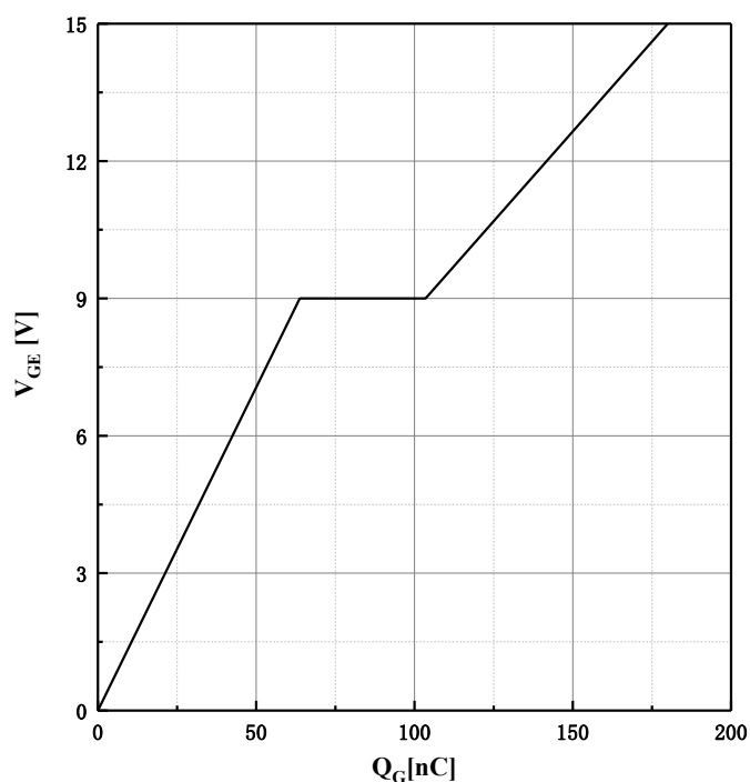
Fig.8 Typical Gate charge V_{GE}=f(Q_G) , I_C=75A , V_{CC}=520V
