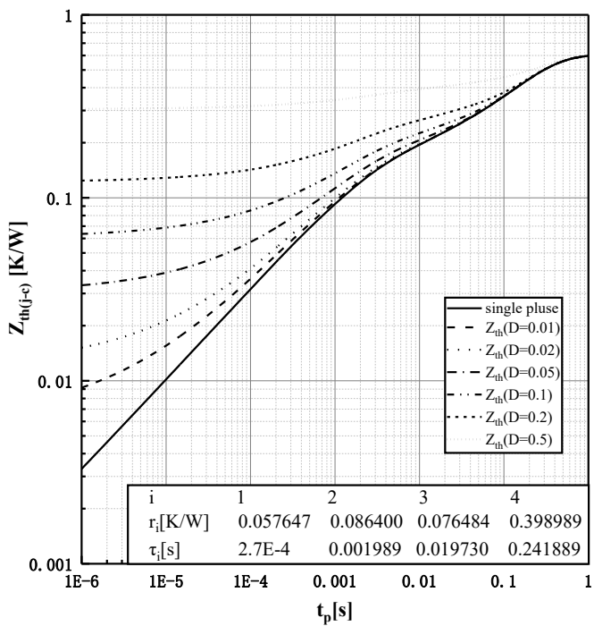
Fig.14 Transient thermal impedance of Diode Z_{th(j-c)}=f(t_p) , D=t_p/T
