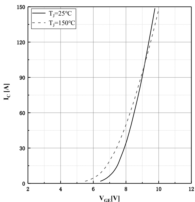
Fig.3 Typical transfer characteristic I_C=f(V_{GE}) , V_{CE}=20\text{V}
