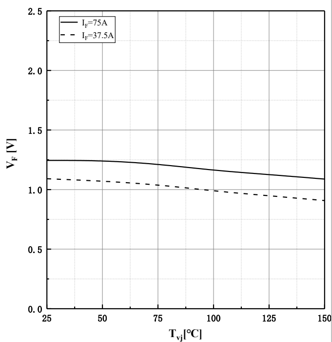
Fig.7 Typical V_F as a function of T_{vj} V_F=f(T_{vj})
