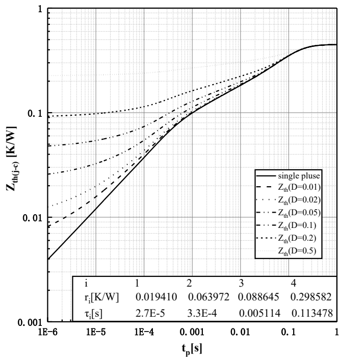
Fig.13 Transient thermal impedance of IGBT Z_{th(j-c)}=f(t_p) , D=t_p/T
