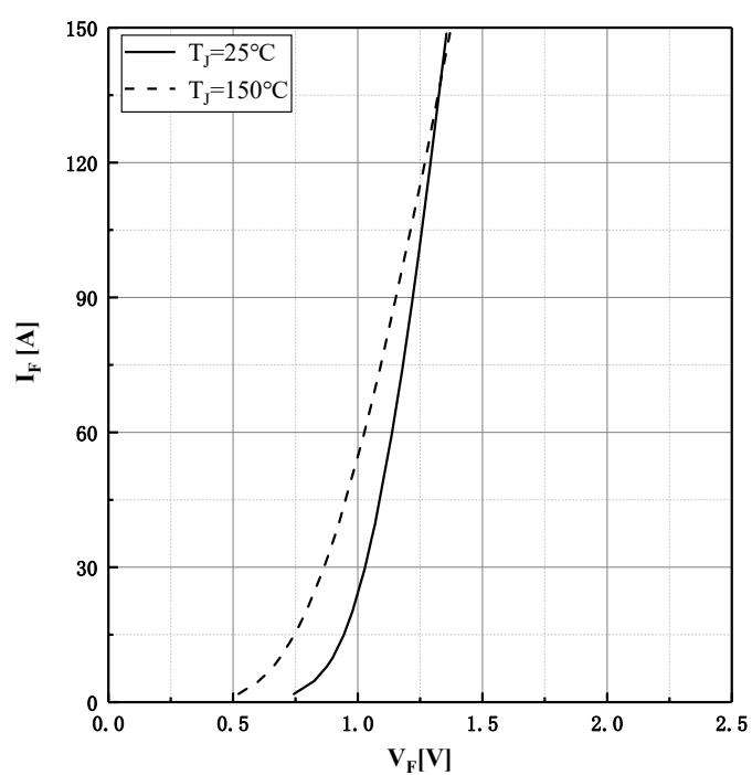
Fig.4 Typical I_F as a function of V_F I_F=f(V_F)
