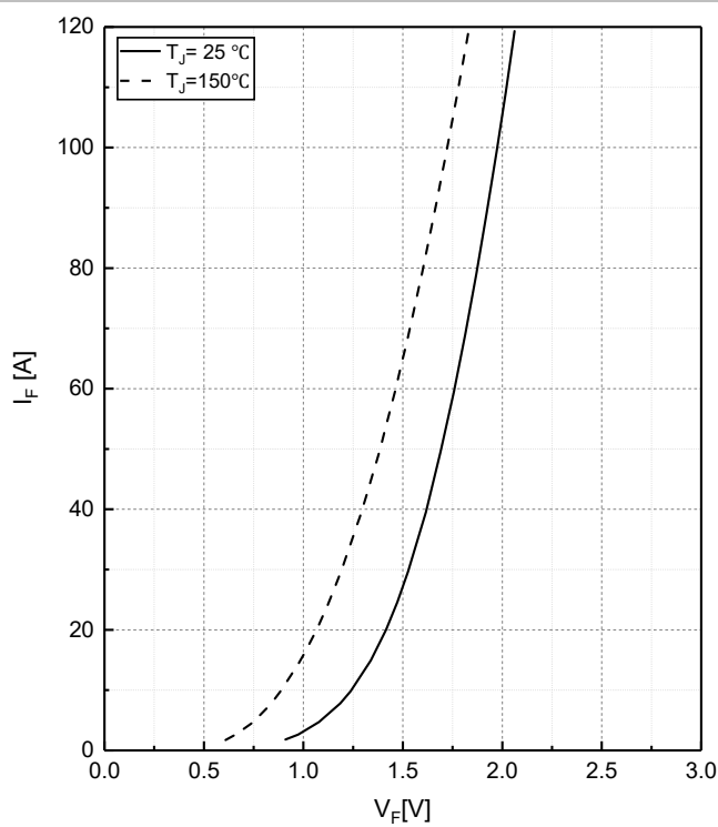
Fig.4 Typical I_F as a function of V_F
