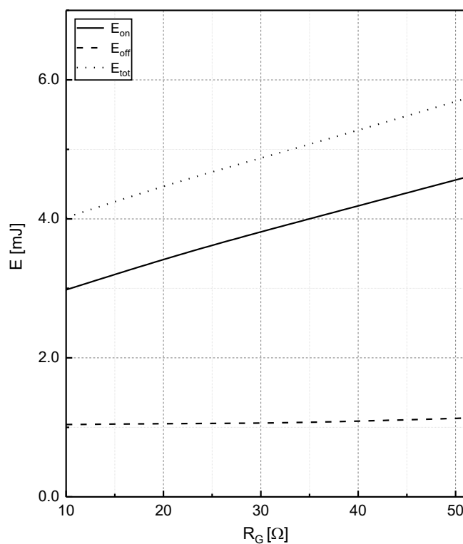
Fig.8 Typical switching loss energy as a function of R_G E=f(R_G), V_{CC}=400V, I_C=60A, V_{GE}=0/15V, T_J=150^\circ C
