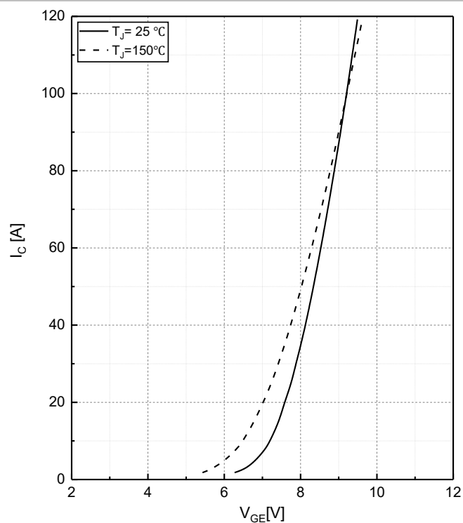
Fig.3 Typical transfer characteristic
