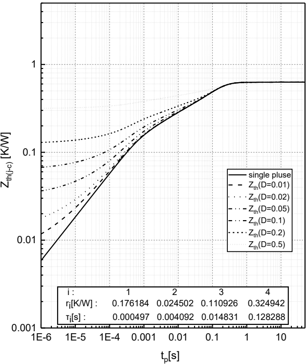
Fig.13 Transient thermal impedance of IGBT Z_{th(j-c)}=f(t_p) , D=t_p/T
