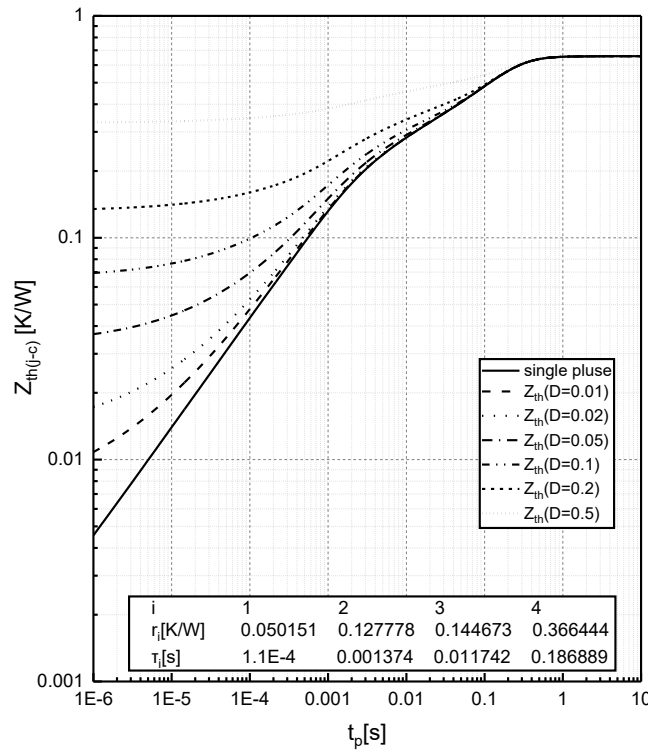
Fig.14 Transient thermal impedance of Diode Z_{th(j-c)}=f(t_p) , D=t_p/T
