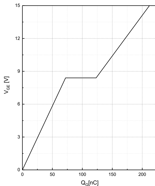
Fig.8 Typical Gate charge V_{GE}=f(Q_G) , I_C=50A , V_{CC}=520V
