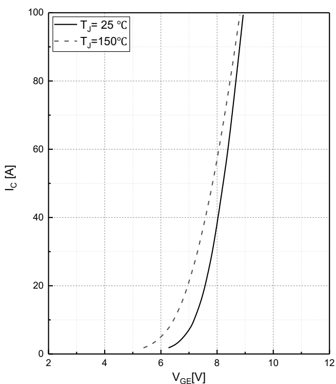
Fig.3 Typical transfer characteristic I_C = f(V_{GE}) , V_{CE} = 20V
