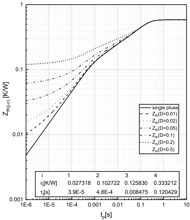
Fig.13 Transient thermal impedance of IGBT Z_{th(j-c)}=f(t_p) , D=t_p/T
