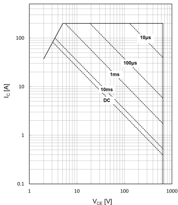
Fig.12 Forward bias safe operating area of IGBT
