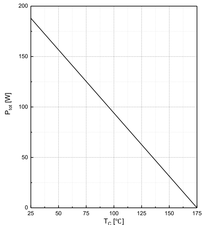
Fig.12 Power dissipation as a function of T_C P_{tot}=f(T_C), T_{vj}\leq 175^{\circ}C, TO-263/TO-220
