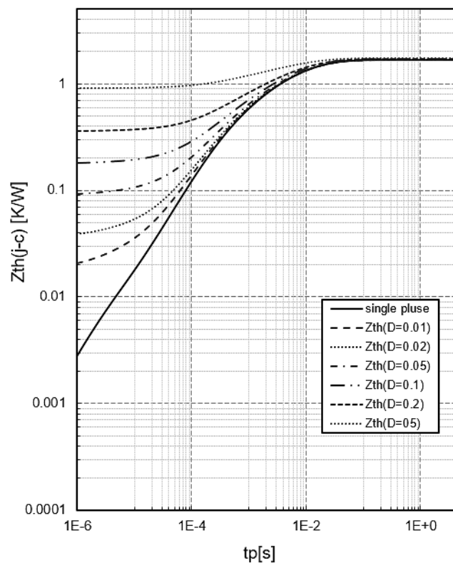
Fig.16 Transient thermal impedance of Diode Z_{th(j-c)}=f(t_p) , D=t_p/T , TO-263/TO-220
