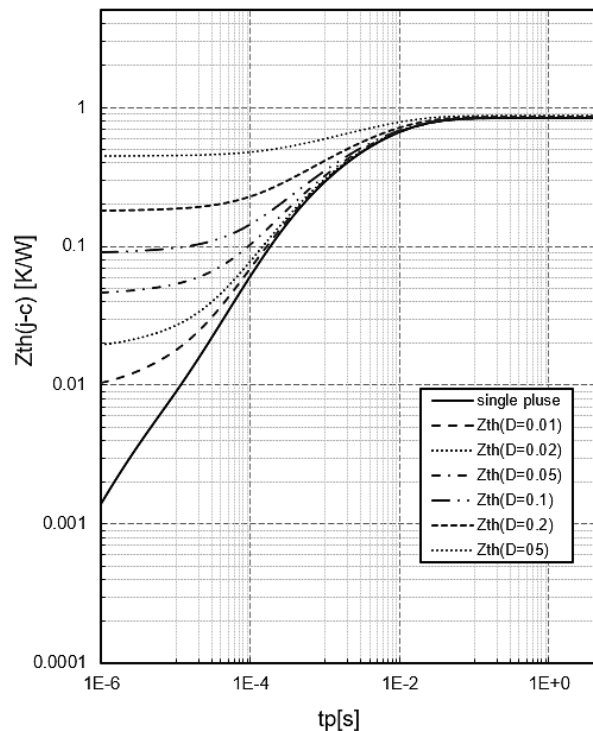
Fig.20 Transient thermal impedance of Diode Z_{th(j-c)}=f(t_p) , D=t_p/T , TO-247
