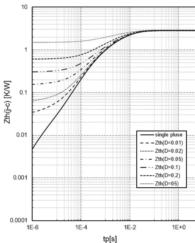
Fig.19 Transient thermal impedance of IGBT Z_{th(j-c)}=f(t_p) , D=t_p/T , TO-247
