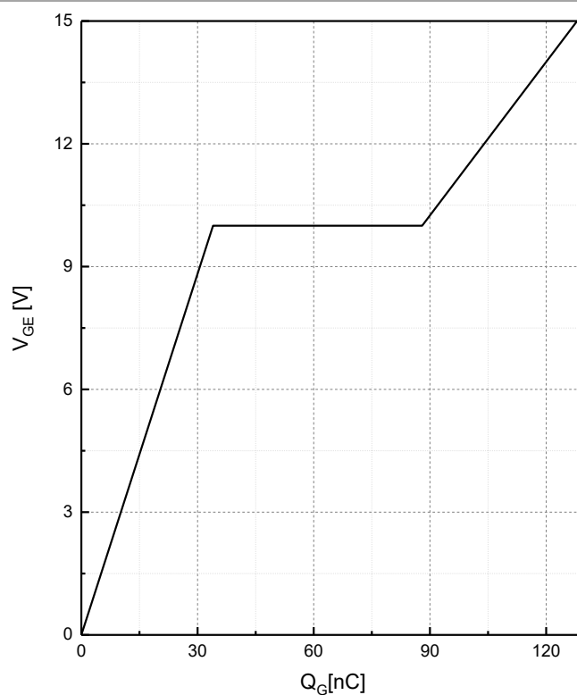
Fig.8 Typical Gate charge V_{GE}=f(Q_G) , I_C=30A
