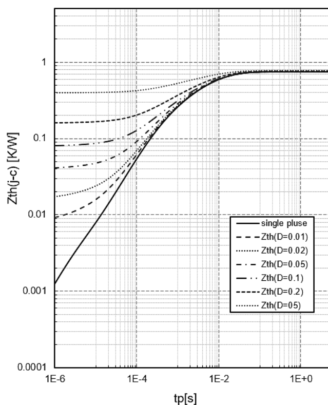
Fig.15 Transient thermal impedance of IGBT Z_{th(j-c)}=f(t_p) , D=t_p/T , TO-263/TO-220
