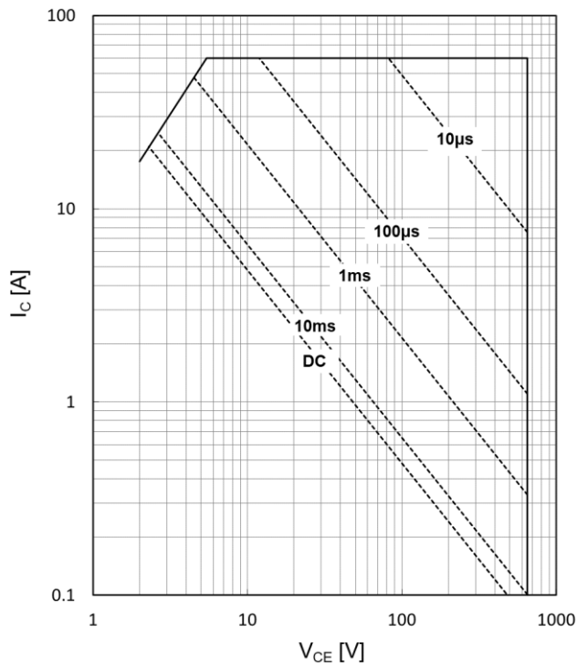
Fig.19 Forward bias safe operating area of IGBT T_c=25^\circ\text{C} , T_{vj}\leq 175^\circ\text{C} , V_{GE}=15\text{V} , single pluse, TO-247
