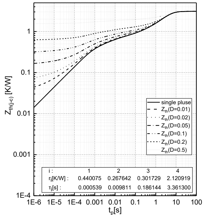
Fig.20 Transient thermal impedance of IGBT Z_{th(j-c)}=f(t_p) , D=t_p/T , TO-247
