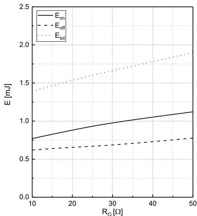
Fig.8 Typical switching loss energy as a function of R_G E=f(R_G) , V_{CC}=400V , I_C=20A , V_{GE}=0/15V , T_J=150°C
