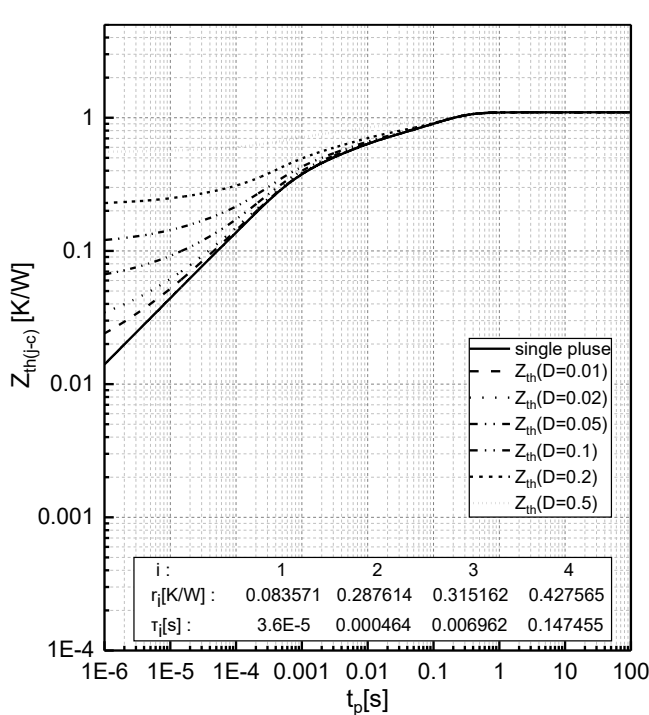
Fig.16 Transient thermal impedance of IGBT Z_{th(j-c)}=f(t_p) , D=t_p/T , TO-263/TO-220
