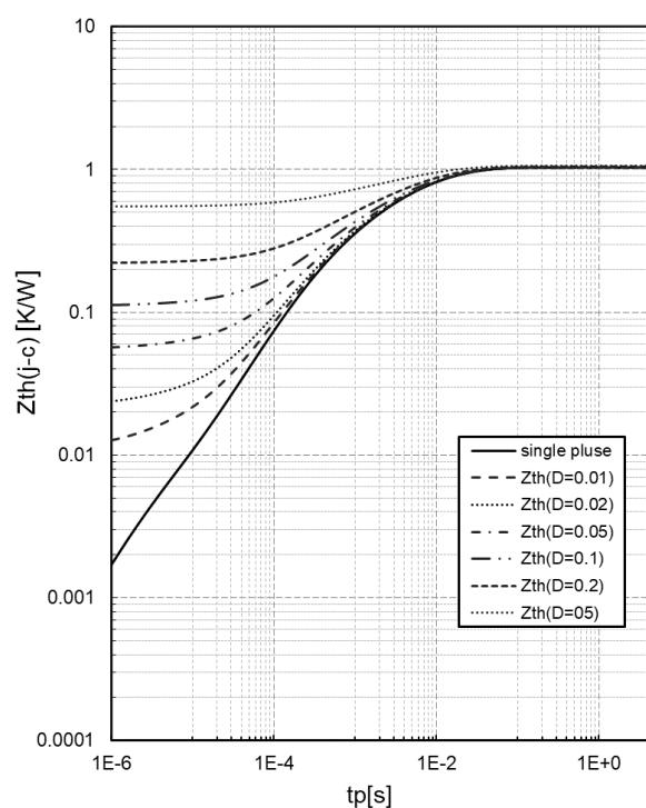
Fig.16 Transient thermal impedance of IGBT Z_{th(j-c)}=f(t_p) , D=t_p/T , TO-252
