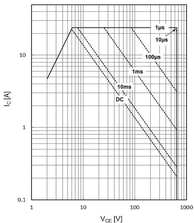
Fig.15 Forward bias safe operating area of IGBT T_c=25^{\circ}\text{C} , T_{vj}\leq 175^{\circ}\text{C} , V_{GE}=15\text{V} , TO-252
