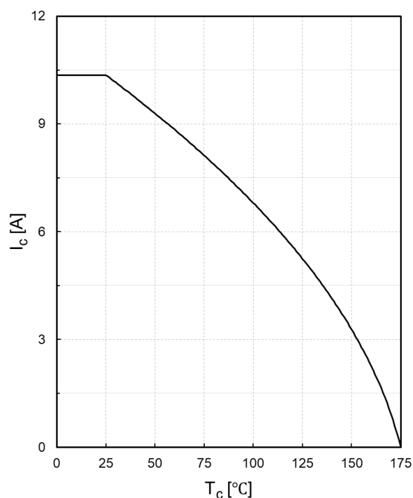
Fig.14 Collector current as a function of case temperature I_c=f(T_{vj}) , TO-220F
