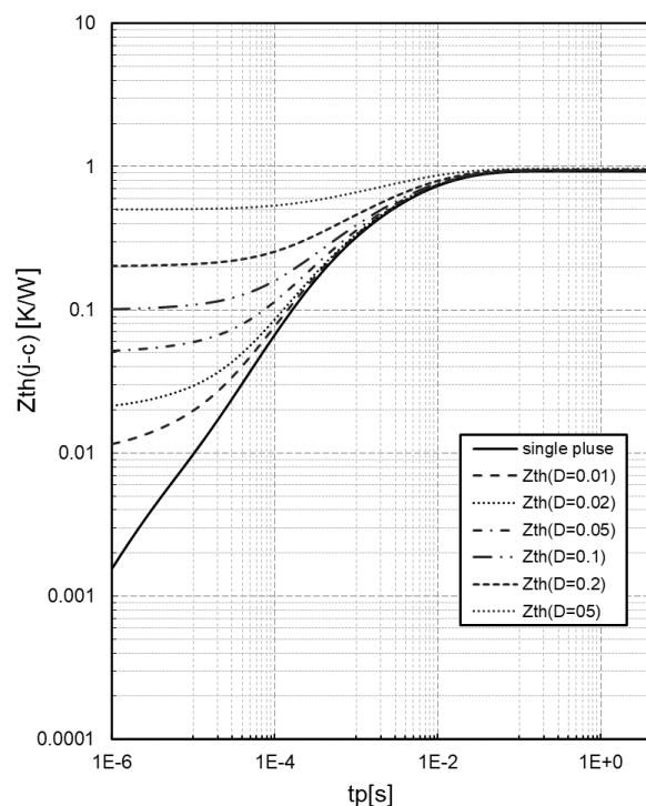
Fig.20 Transient thermal impedance of IGBT
