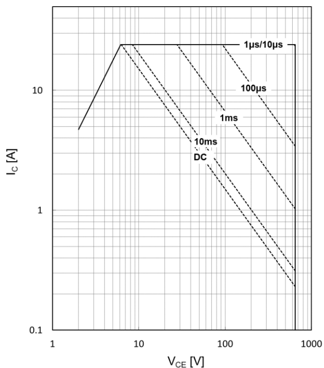
Fig.19 Forward bias safe operating area of IGBT
