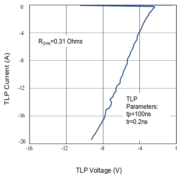
Figure 6: TLP Negative I-V Curve
