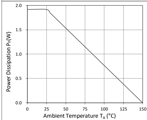
Figure 9. Power Dissipation
