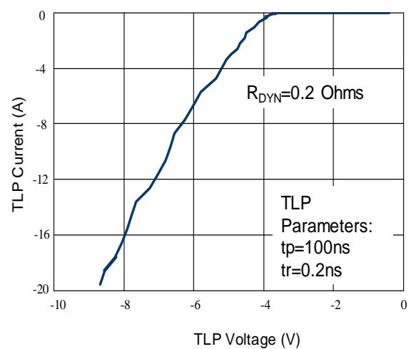
Figure 6: TLP Negative I-V Curve
